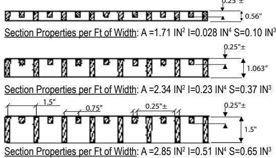
Elevation View
